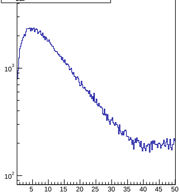
t-t_{\text{ear}} , nHits/tray/ev>25
