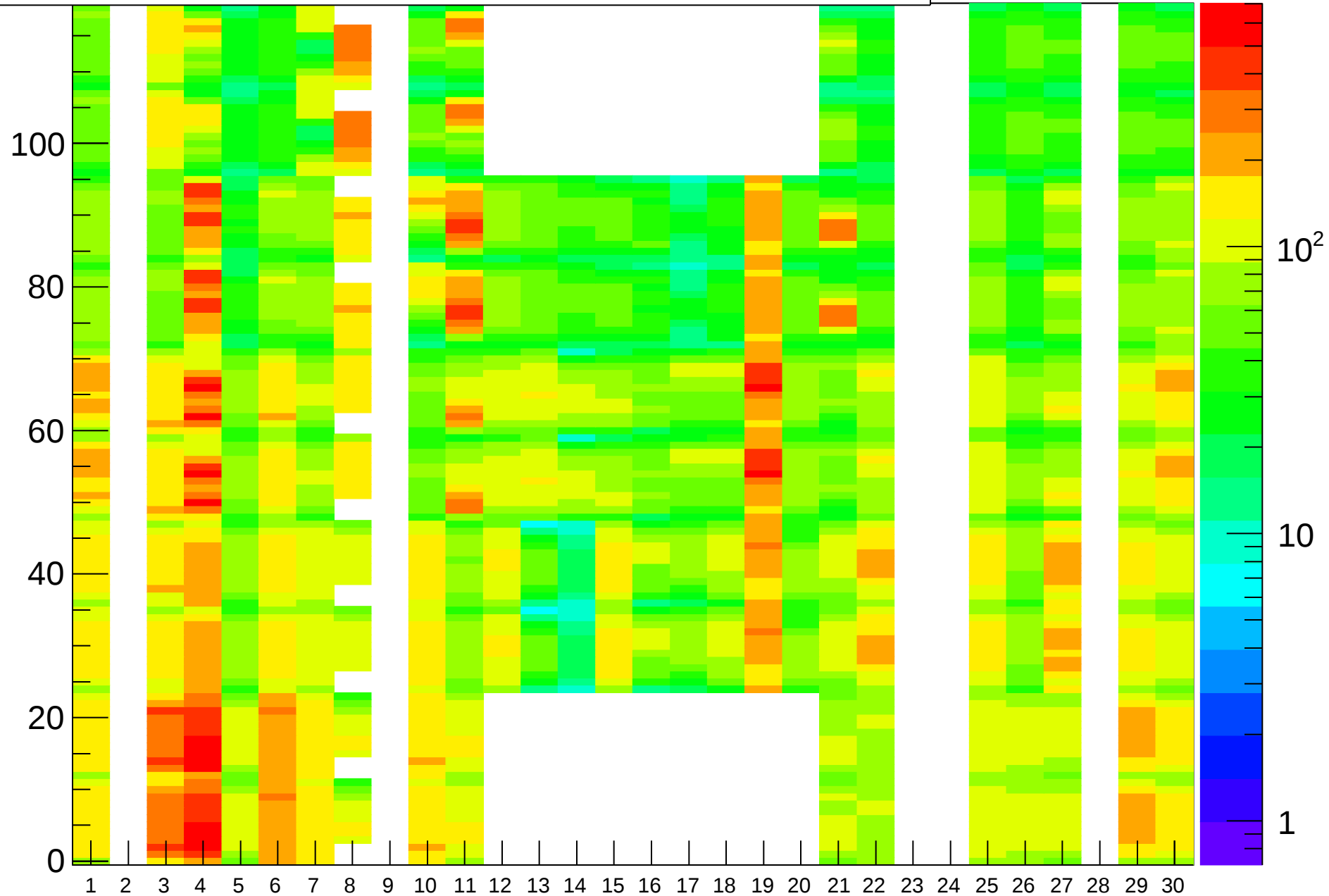
Rate (Hz) vs (BL,strip-posn), Run=26163
