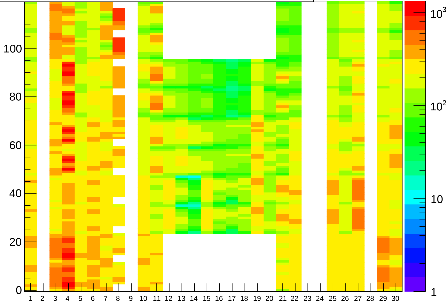
Rate (Hz) vs (BL,strip-posn), Run=26194
