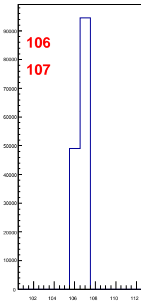
hbunchidoffset_thubhalf41
