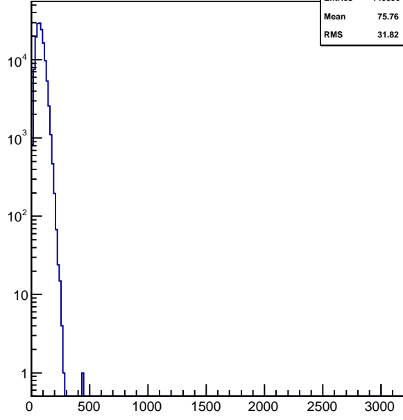
hnhitstof_xingp2_vpd
