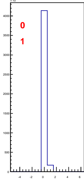
hbunchidoffset_thubhalf11
