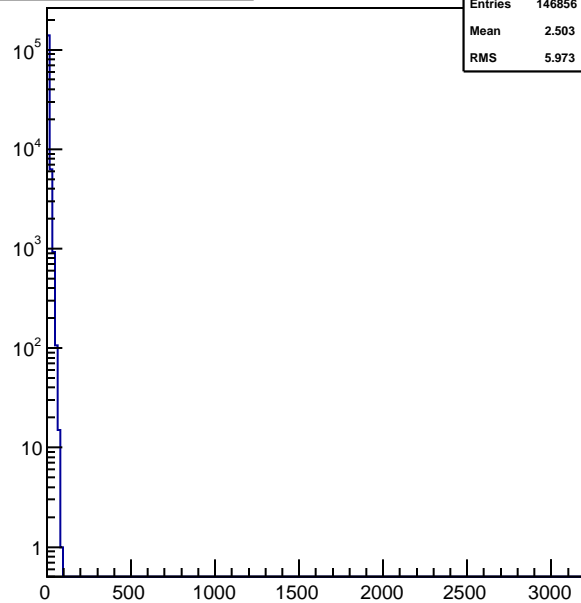
hnhitstof_xingm7
