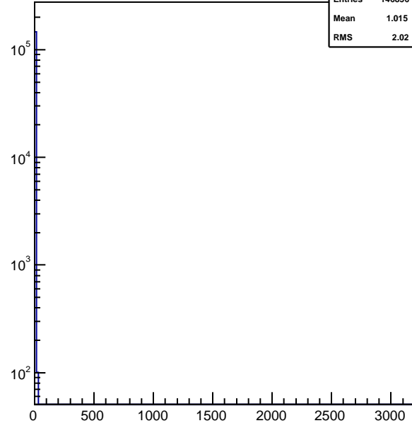
hnhitstof_xingm7_vpd
