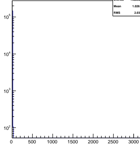
hnhitstof_xingp7_vpd
