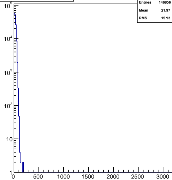
hnhitstof_xingm7
