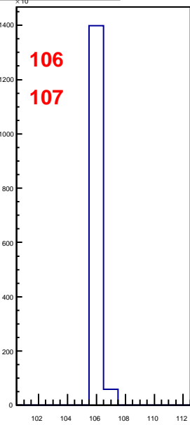
hbunchidoffset_thubhalf51
