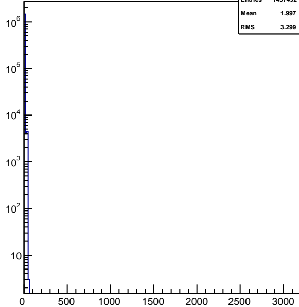
hnhitstof_xingp7_vpd
