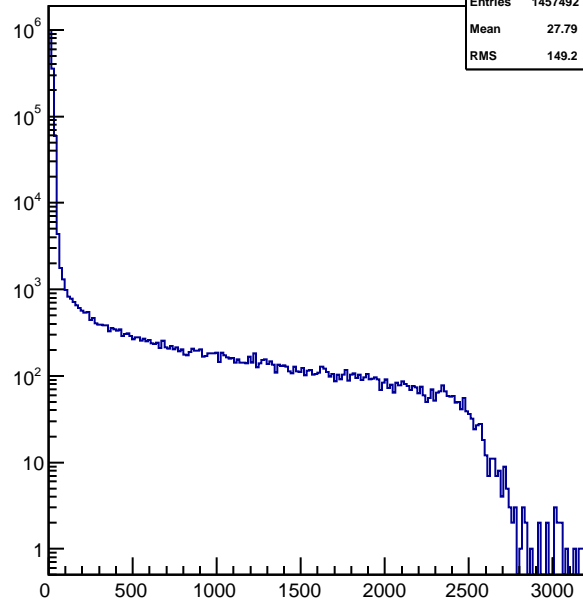
hnhitstof_xingp7
