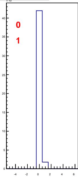
hbunchidoffset_thubhalf11
