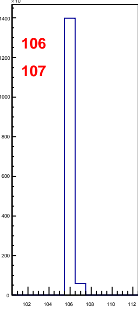
hbunchidoffset_thubhalf50
