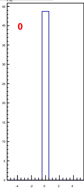
hbunchidoffset_thubhalf21
