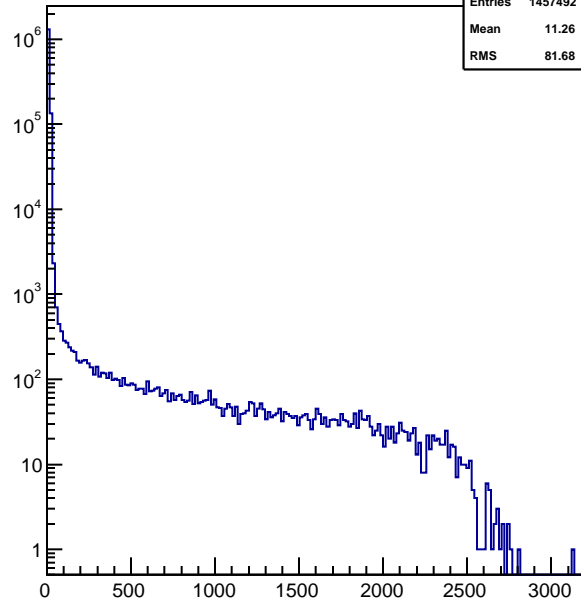
hnhitstof_xingm7
