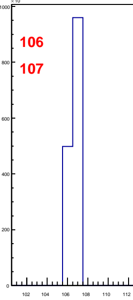
hbunchidoffset_thubhalf40
