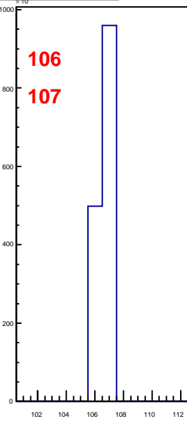
hbunchidoffset_thubhalf41
