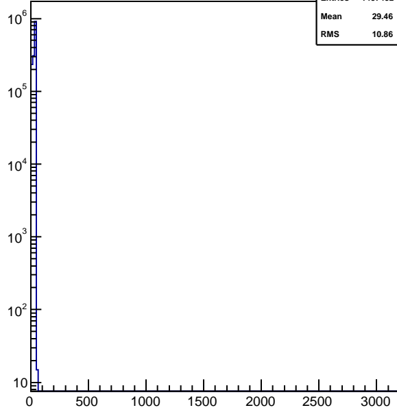
hnhitstof_xingm7_vpd
