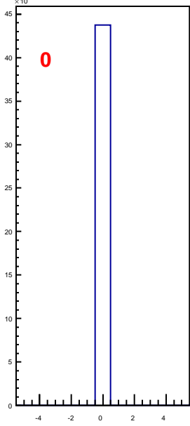
hbunchidoffset_thubhalf20
