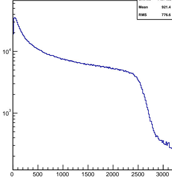
hnhitstof_xingp2_vpd
