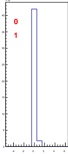
hbunchidoffset_thubhalf10
