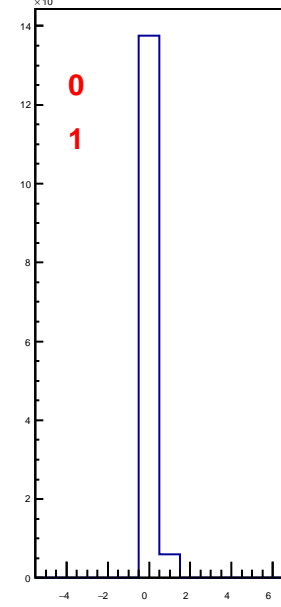
hbunchidoffset_thubhalf10
