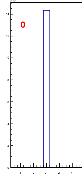
hbunchidoffset_thubhalf20
