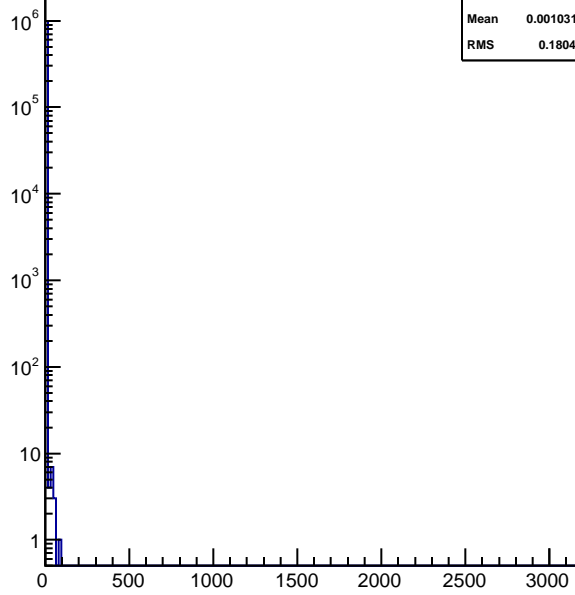
hnhitstof_xingp2_vpd
