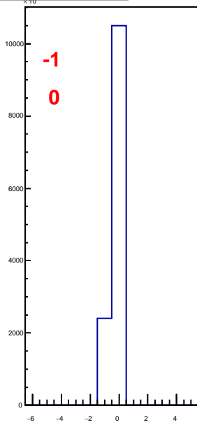
hbunchidoffset_thubhalf31
