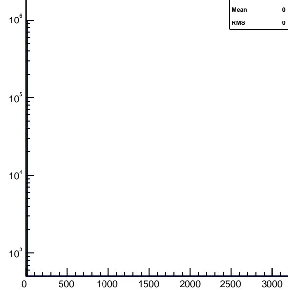
hnhitstof_xingp7
