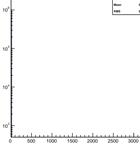
hnhitstof_xingp2
