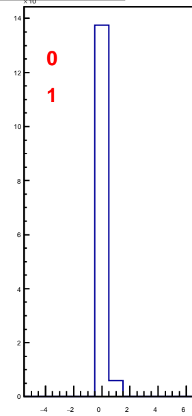
hbunchidoffset_thubhalf11
