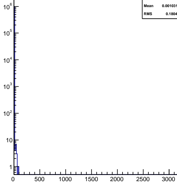
hnhitstof_xingp2
