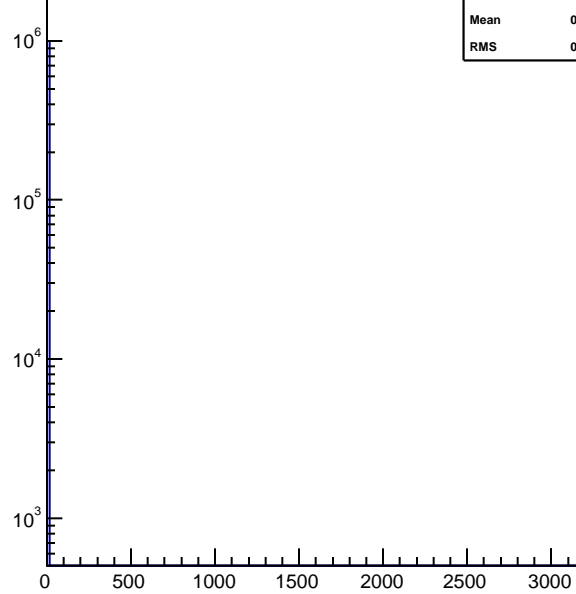
hnhitstof_xingm7
