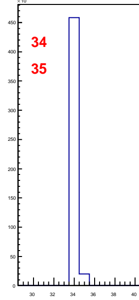
hbunchidoffset_thubhalf50
