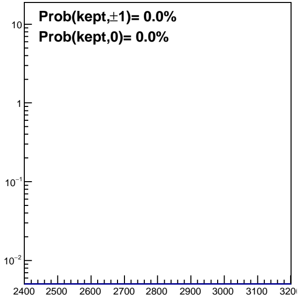
trgdtime, VPD 121
