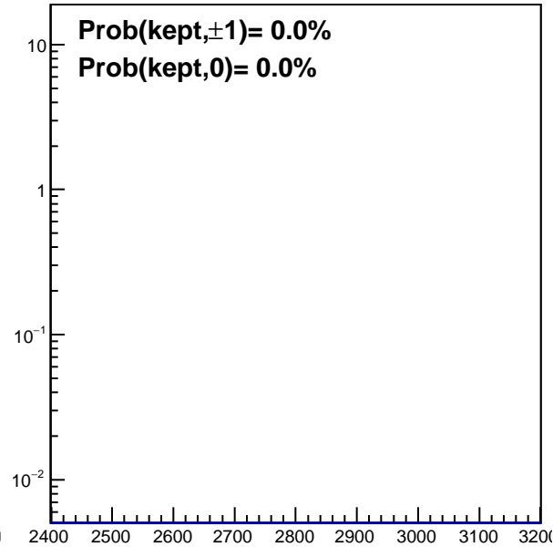
trgdtime, VPD 122
