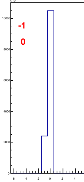
hbunchidoffset_thubhalf30
