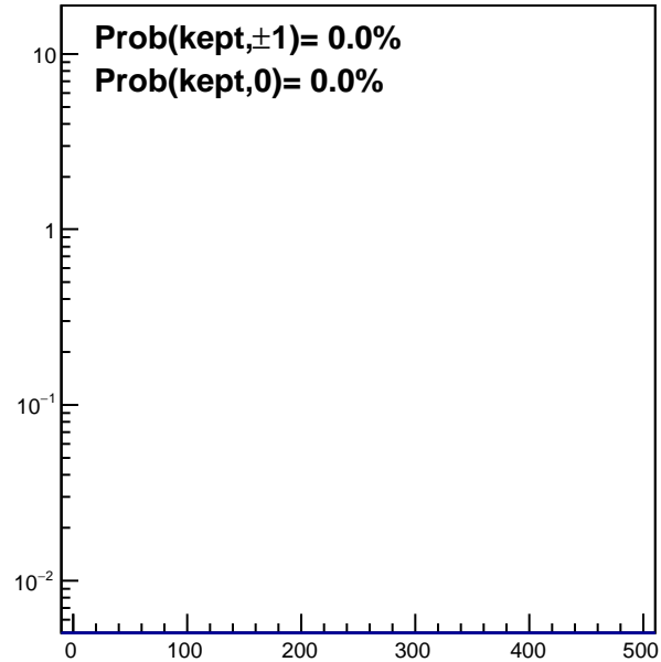
trgdtime, VPD 122
