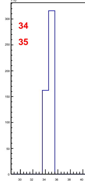
hbunchidoffset_thubhalf40
