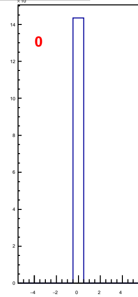
hbunchidoffset_thubhalf21
