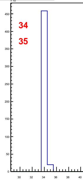
hbunchidoffset_thubhalf51
