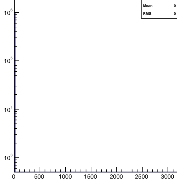
hnhitstof_xingm7_vpd
