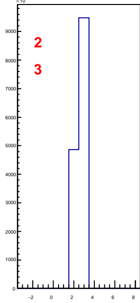
hbunchidoffset_thubhalf00
