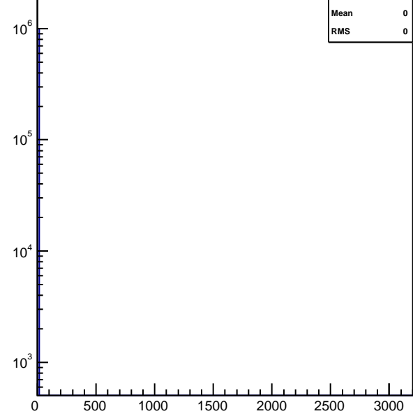
hnhitstof_xingp7_vpd
