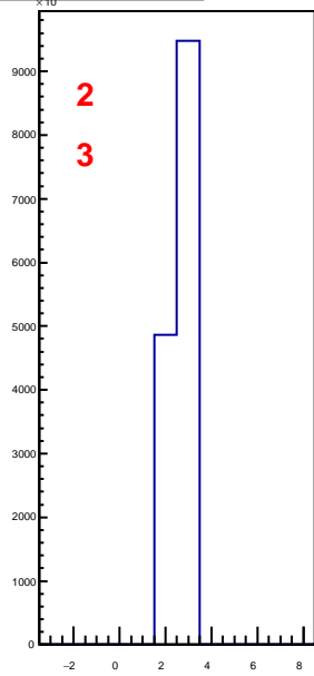
hbunchidoffset_thubhalf01
