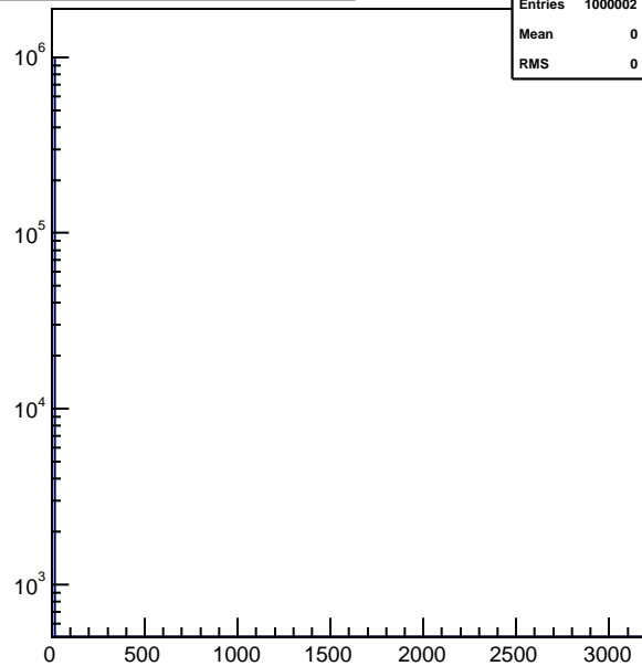
hnhitstof_xingm7_vpd
