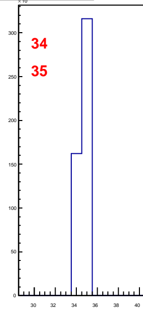
hbunchidoffset_thubhalf41
