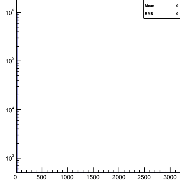
hnhitstof_xingp7
