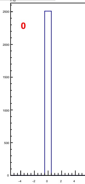
hbunchidoffset_thubhalf21
