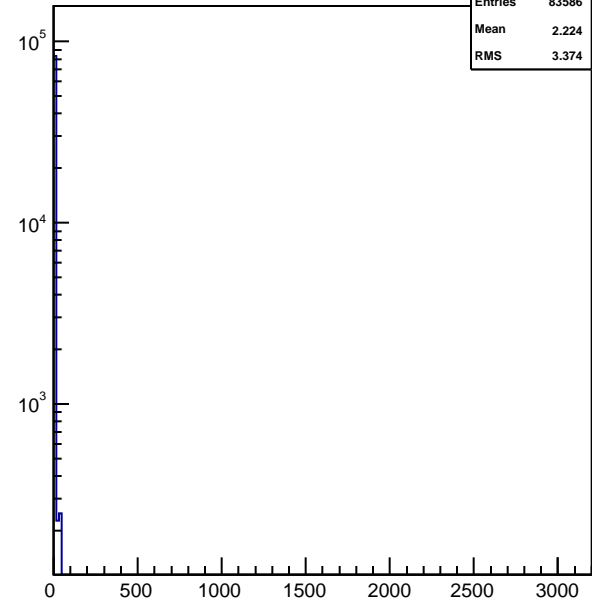
hnhitstof_xingp7_vpd
