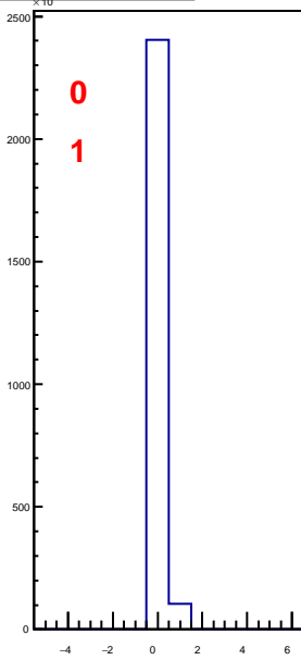
hbunchidoffset_thubhalf11
