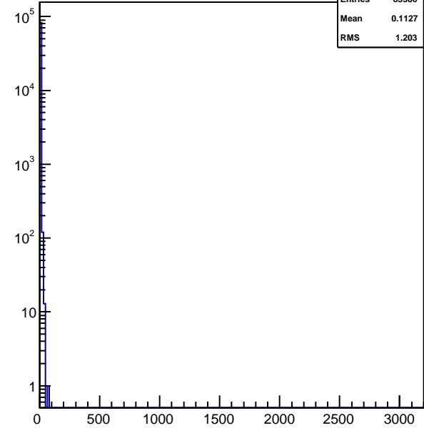
hnhitstof_xingp7
