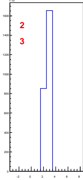
hbunchidoffset_thubhalf00
