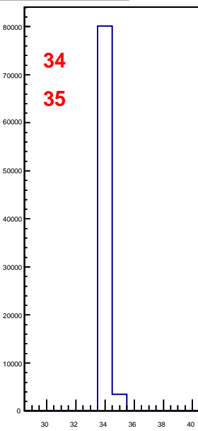
hbunchidoffset_thubhalf51
