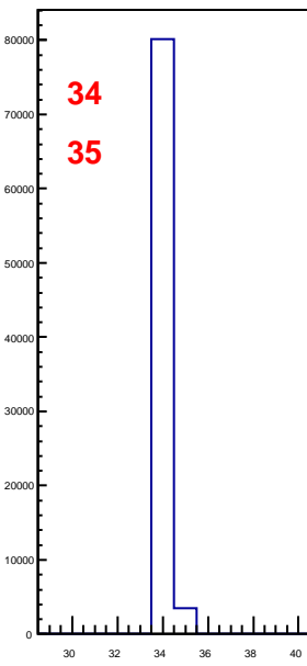
hbunchidoffset_thubhalf50
