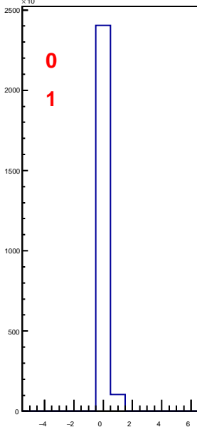
hbunchidoffset_thubhalf10
