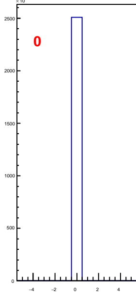
hbunchidoffset_thubhalf20
