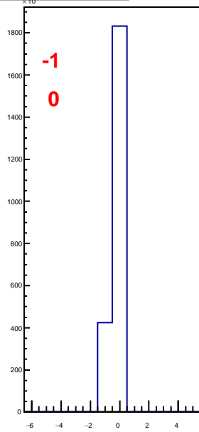
hbunchidoffset_thubhalf31
