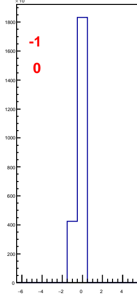
hbunchidoffset_thubhalf30
