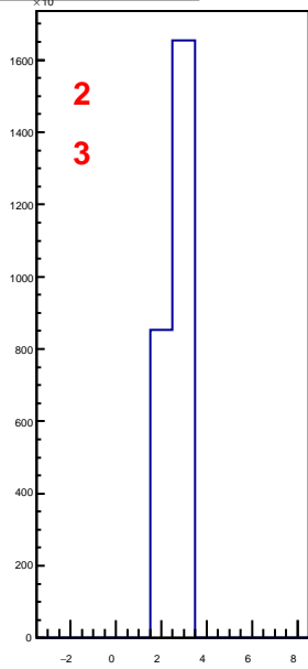
hbunchidoffset_thubhalf01
