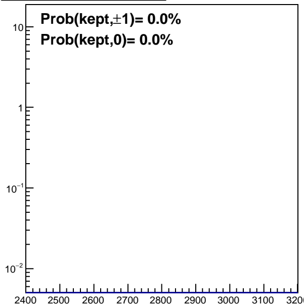
trgdtime, VPD 121
