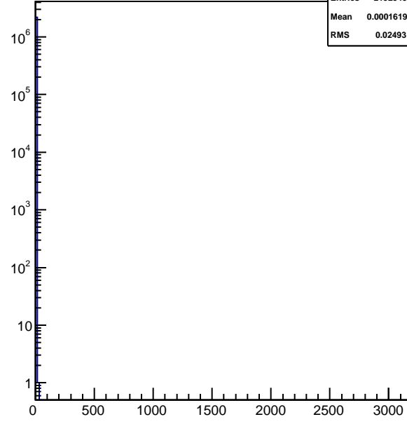
hhhitstof_xingp7
