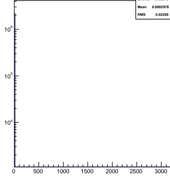
hhhitstof_xingm7
