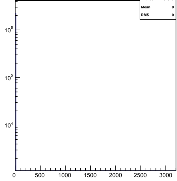
hnhitstof_xingp7_vpd
