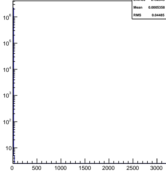
hhhitstof_xingp2
