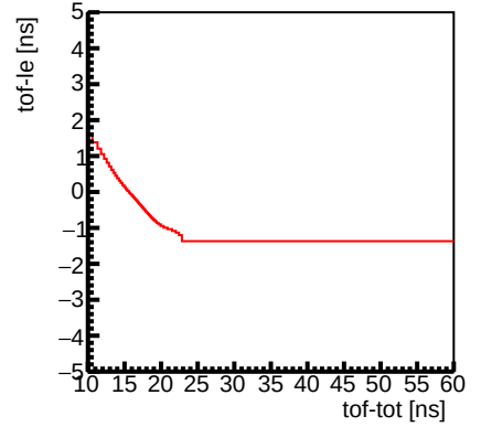
Channel 6 : Slewing Correction
