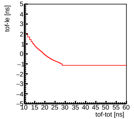
Channel 9 : Slewing Correction
