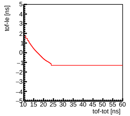
Channel 3 : Slewing Correction
