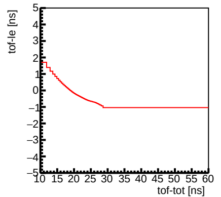
Channel 12 : Slewing Correction
