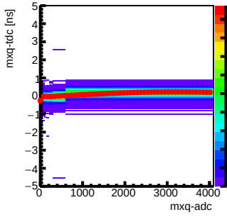
Step 6 : Channel 24 mxq-tdc vs mxq-adc
