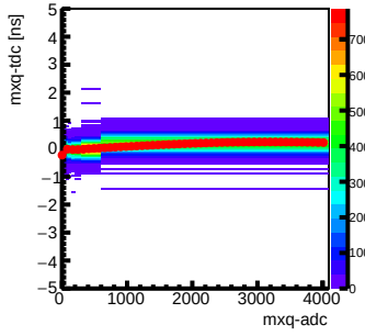
Step 6 : Channel 26 mxq-tdc vs mxq-adc
