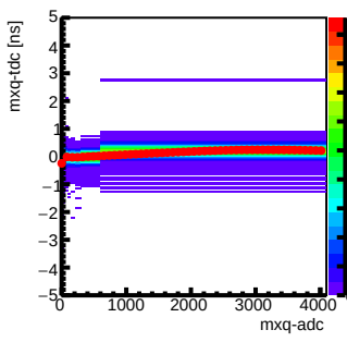
Step 6 : Channel 20 mxq-tdc vs mxq-adc
