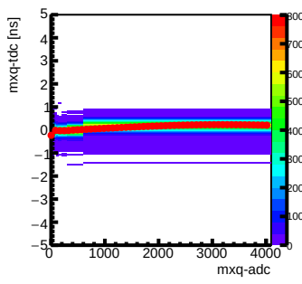
Step 6 : Channel 23 mxq-tdc vs mxq-adc
