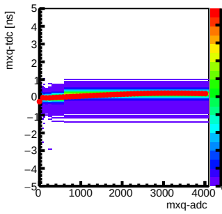
Step 6 : Channel 32 mxq-tdc vs mxq-adc
