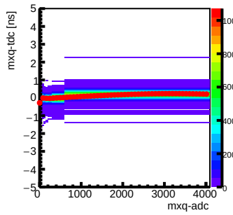
Step 6 : Channel 33 mxq-tdc vs mxq-adc
