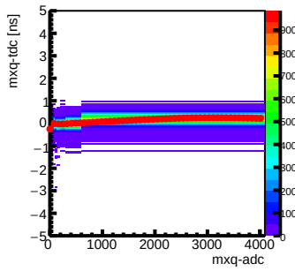
Step 6 : Channel 35 mxq-tdc vs mxq-adc
