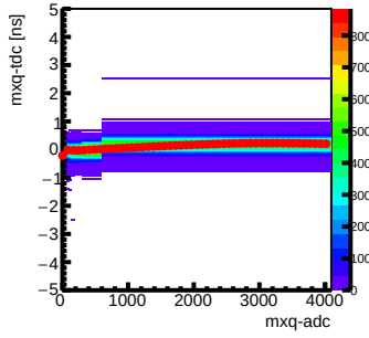
Step 6 : Channel 27 mxq-tdc vs mxq-adc
