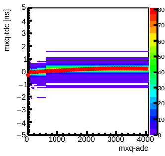
Step 6 : Channel 22 mxq-tdc vs mxq-adc
