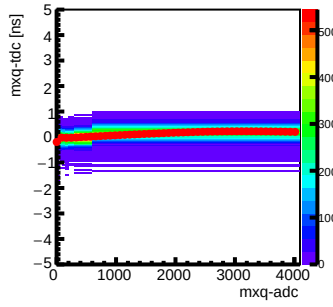
Step 6 : Channel 29 mxq-tdc vs mxq-adc
