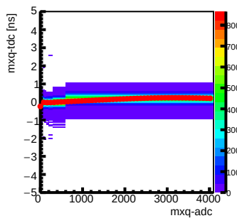
Step 6 : Channel 21 mxq-tdc vs mxq-adc
