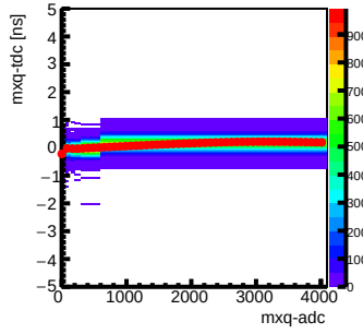
Step 6 : Channel 25 mxq-tdc vs mxq-adc
