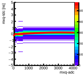
Step 6 : Channel 31 mxq-tdc vs mxq-adc
