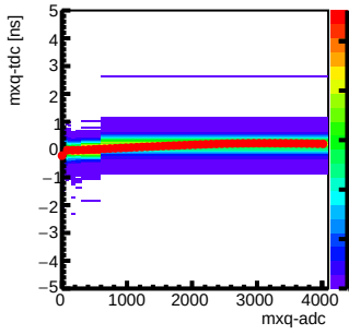
Step 6 : Channel 28 mxq-tdc vs mxq-adc
