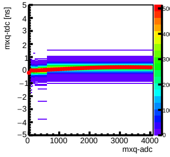
Step 6 : Channel 30 mxq-tdc vs mxq-adc
