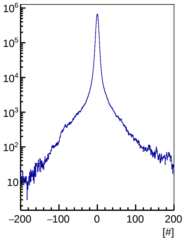
it5z TPC - z VPD
