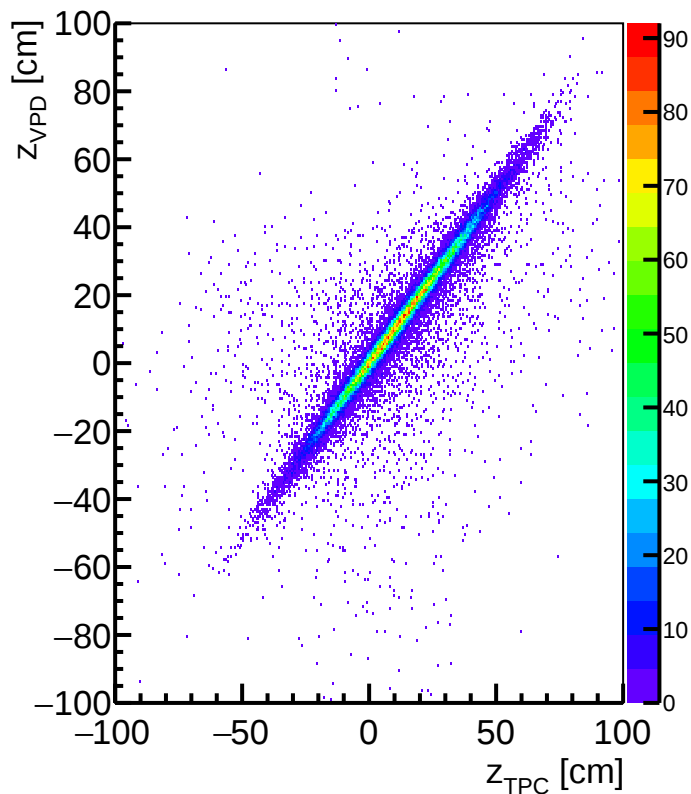
TPC vs. VPD z Vertex using <East> & <West>
