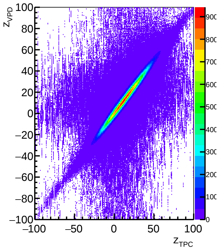
TPC vs. VPD z Vertex
