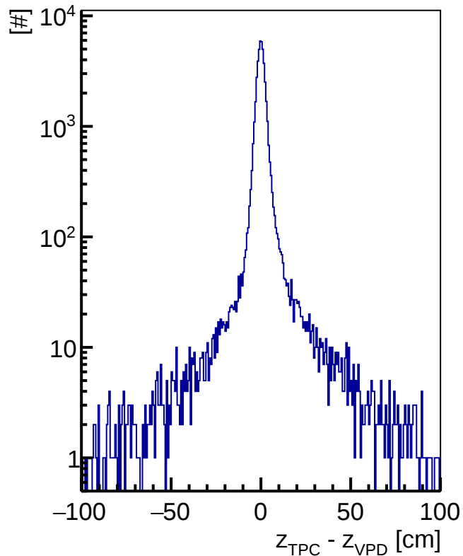
TPC vs. VPD z Vertex using <East> & <West>
