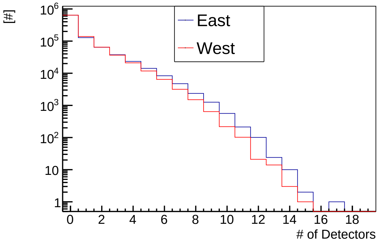
Step 6 : # of Accepted Detectors
