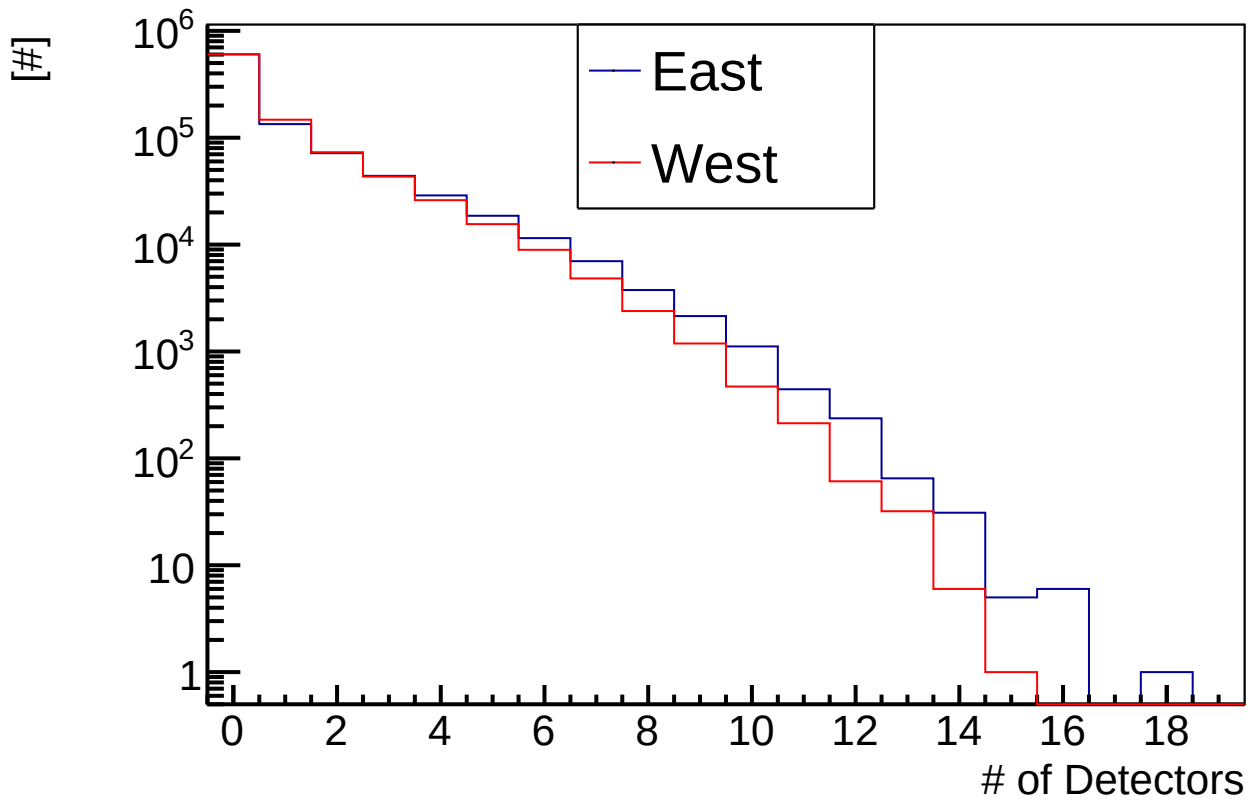
Step 2 : # of Accepted Detectors
