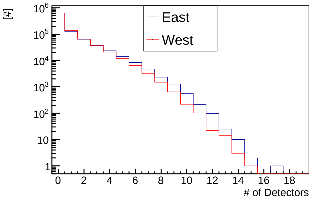
Step 5 : # of Accepted Detectors
