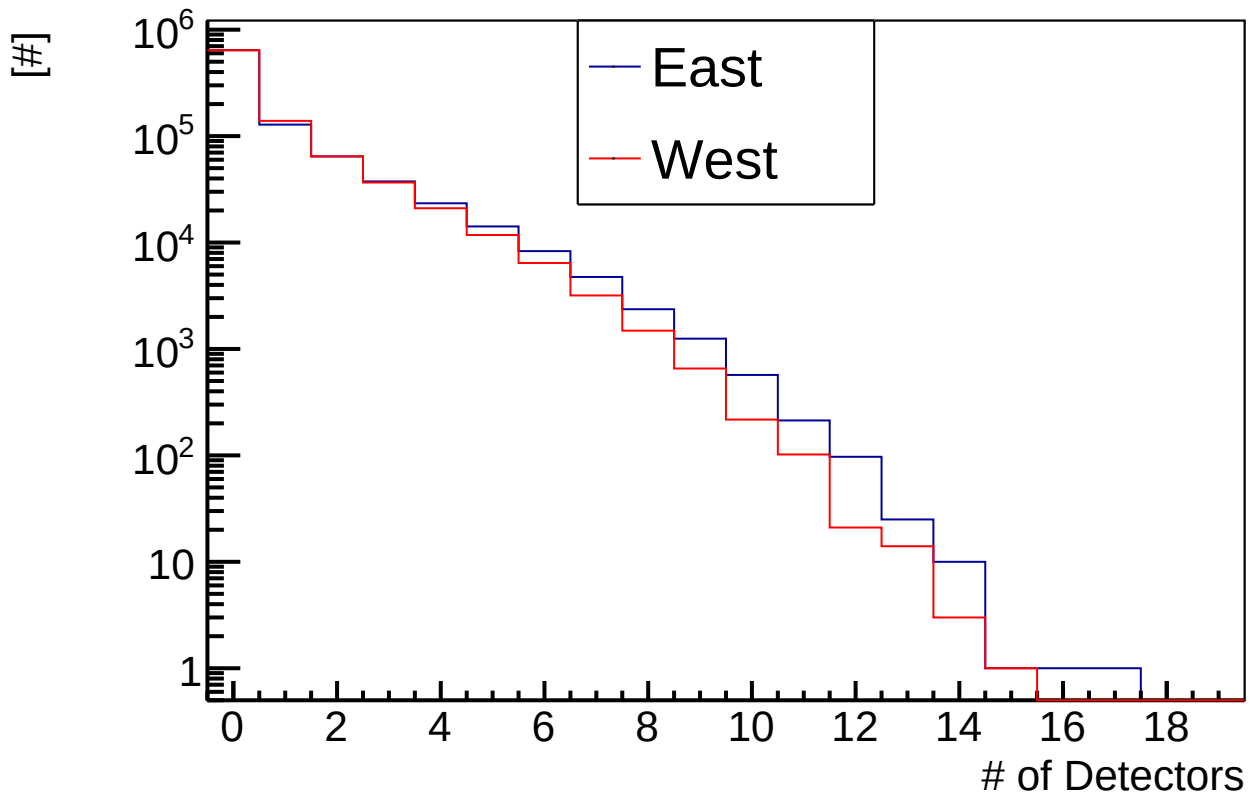
Step 4 : # of Accepted Detectors
