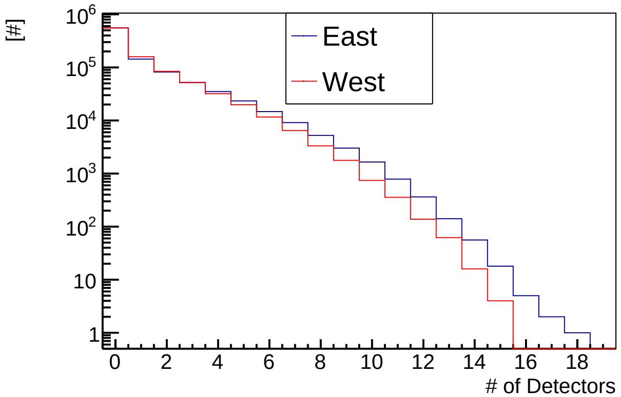
Step 1 : # of Accepted Detectors
