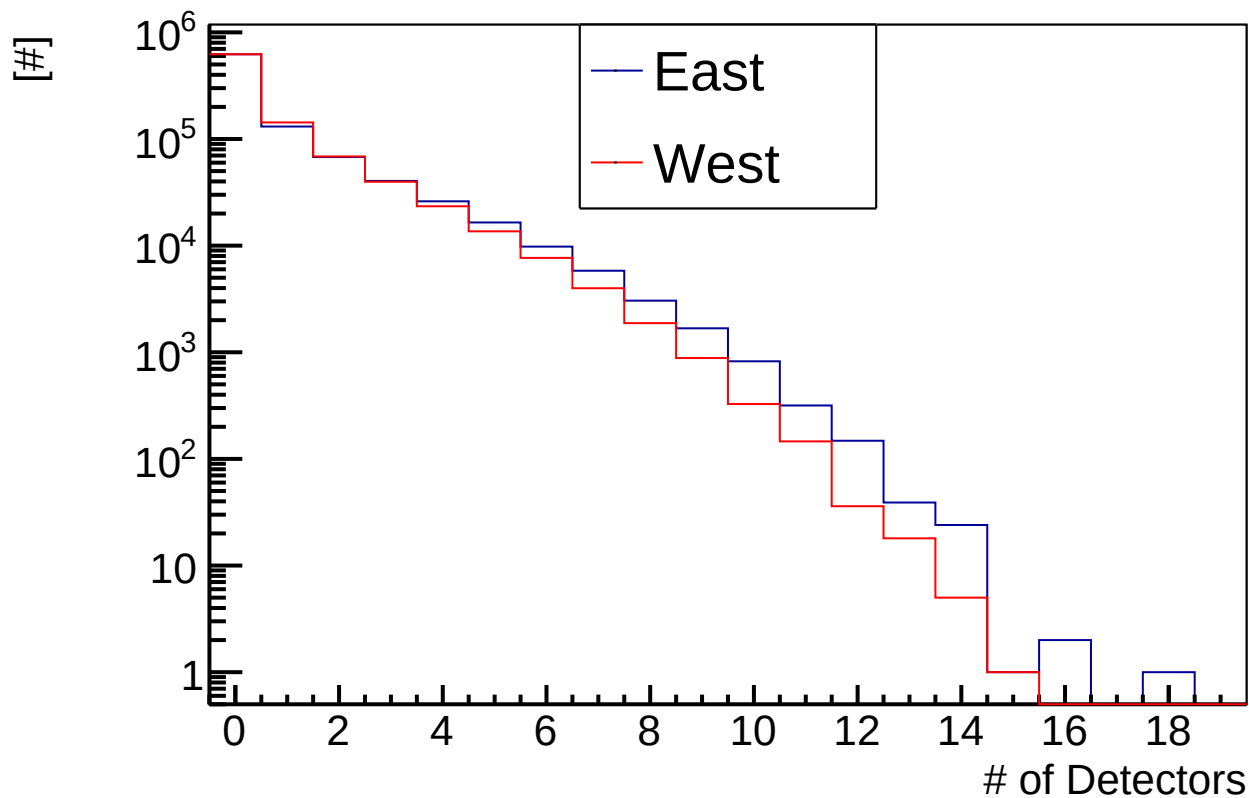
Step 3 : # of Accepted Detectors
