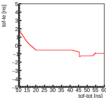
Channel 2 : Slewing Correction
