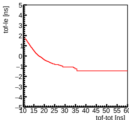
Channel 12 : Slewing Correction
