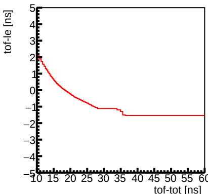
Channel 5 : Slewing Correction
