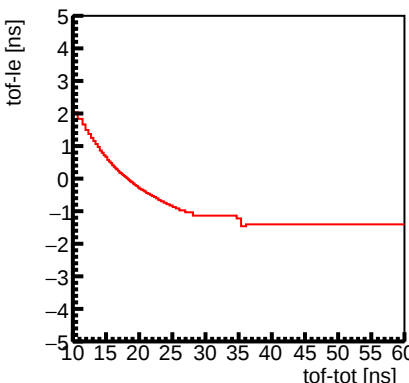
Channel 10 : Slewing Correction
