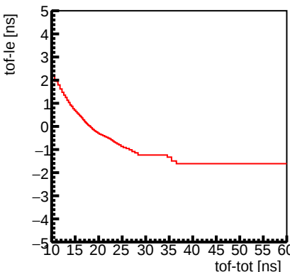
Channel 4 : Slewing Correction
