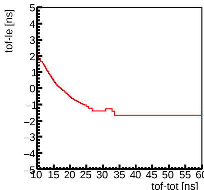
Channel 6 : Slewing Correction
