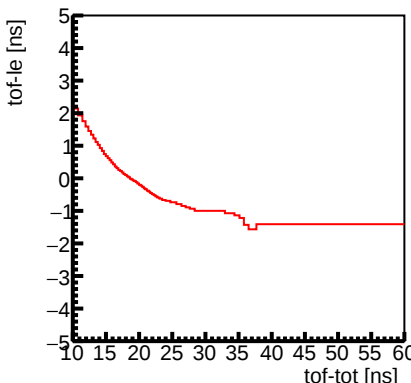
Channel 8 : Slewing Correction
