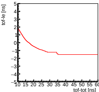
Channel 1 : Slewing Correction
