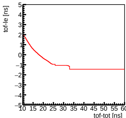
Channel 3 : Slewing Correction
