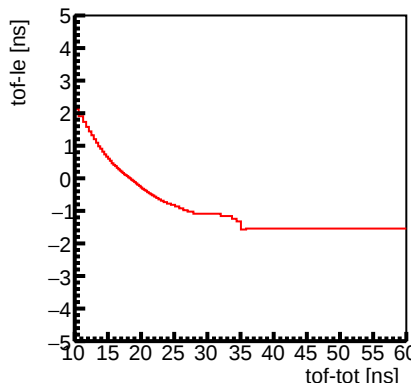
Channel 9 : Slewing Correction
