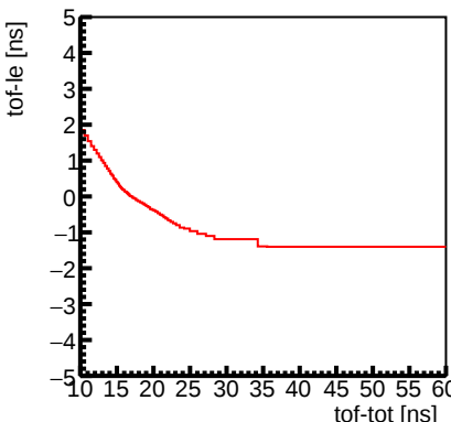
Channel 7 : Slewing Correction
