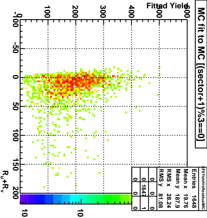
MC fit to Data [(sector+1)%3==0]
