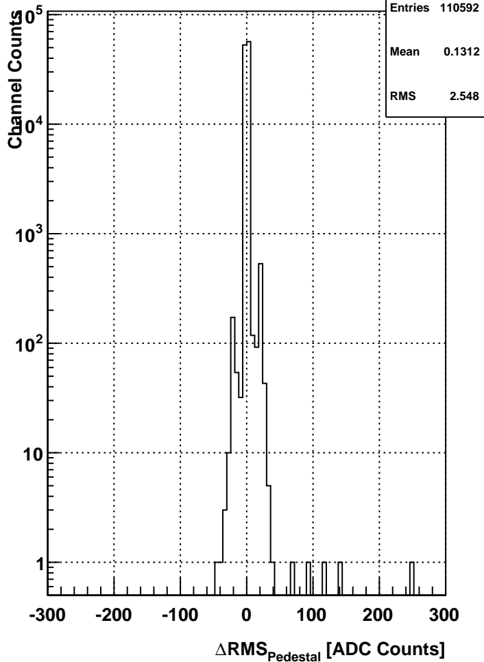
hist_rmsPedDiff_TimeBin1_1D
