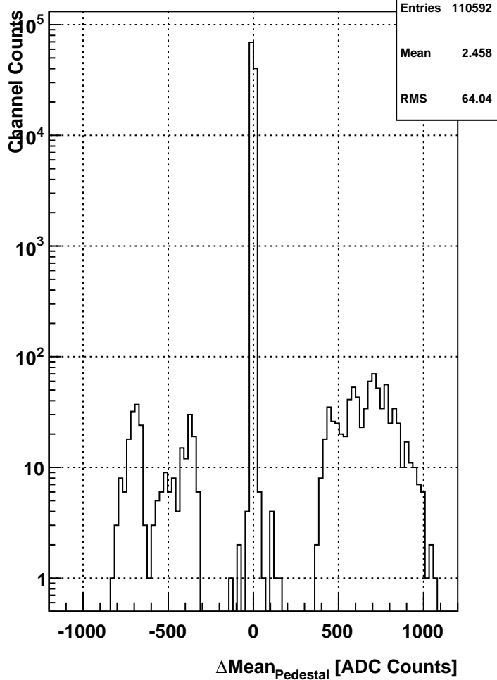
hist_meanPedDiff_TimeBin1_1D
