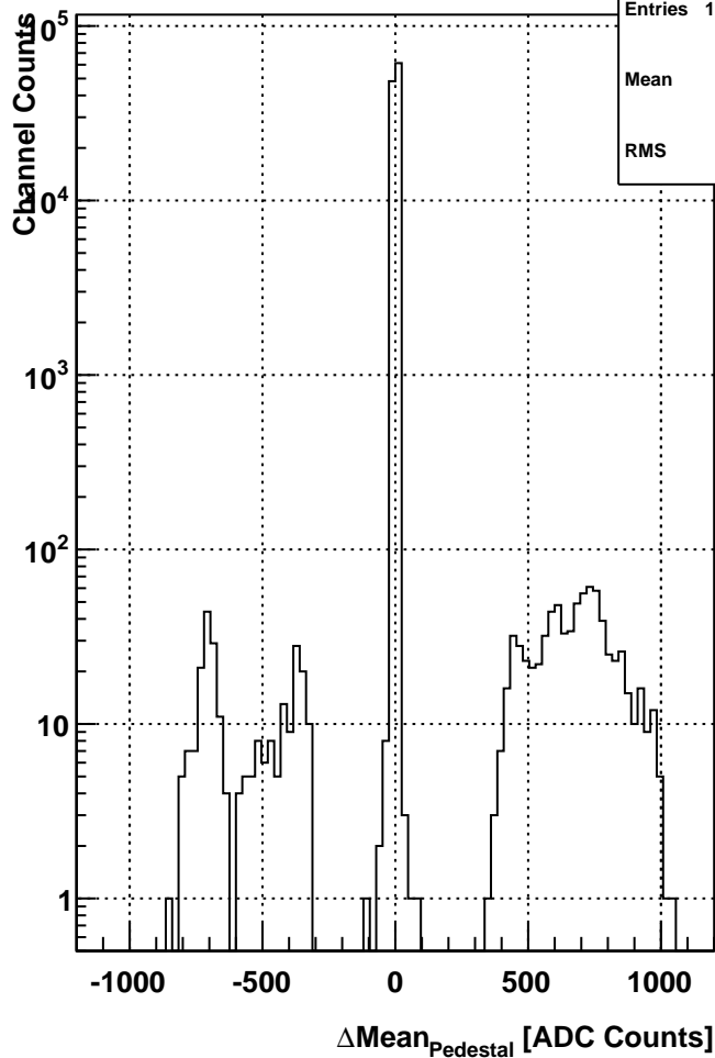
hist_meanPedDiff_TimeBin8_1D
