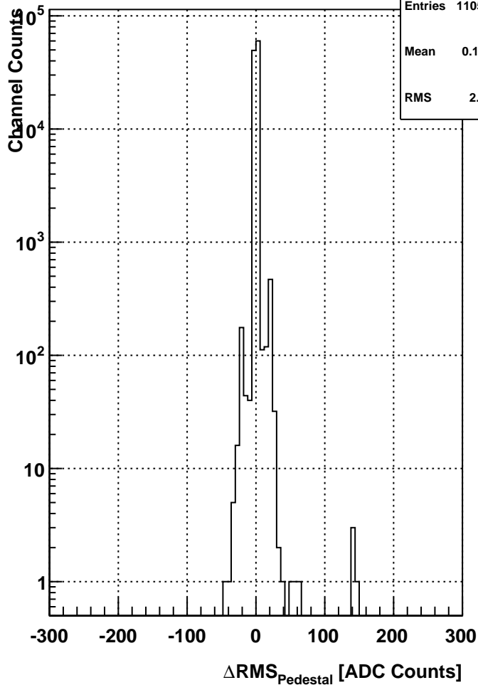
hist_rmsPedDiff_TimeBin8_1D
